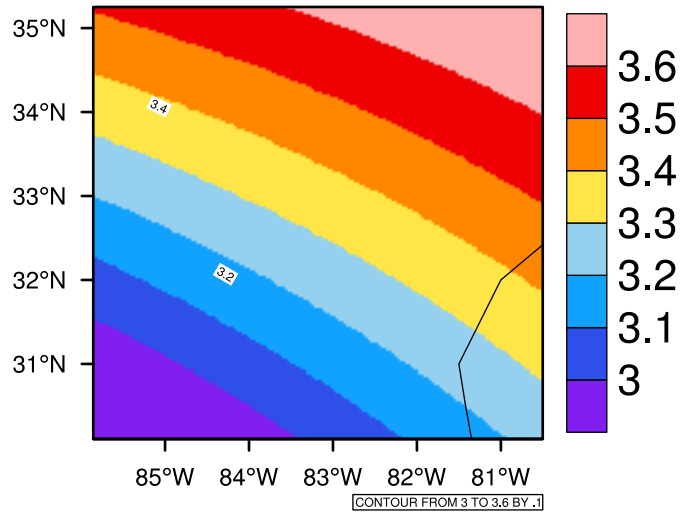
Yearly pr (mm/day) In 2060-2069 GFDL-ESM2M RCP45 - Georgia
