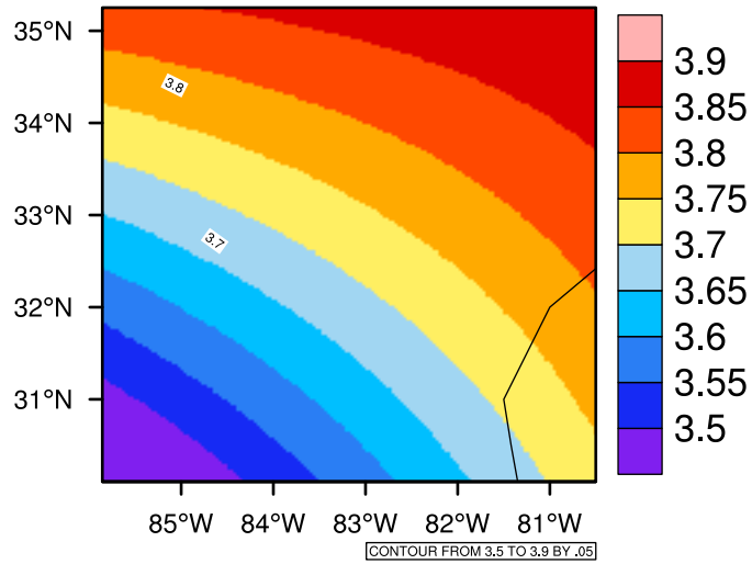
Yearly pr (mm/day) In 2080-2089 GFDL-ESM2M RCP45 - Georgia
