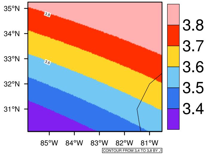
Yearly pr (mm/day) In 2030-2039 GFDL-ESM2M RCP85 - Georgia
