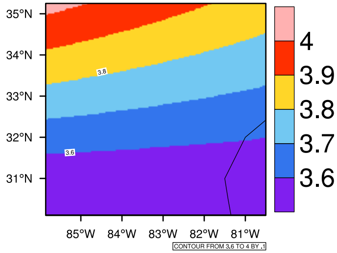
Yearly pr (mm/day) In 2040-2049 GFDL-ESM2M RCP85 - Georgia
