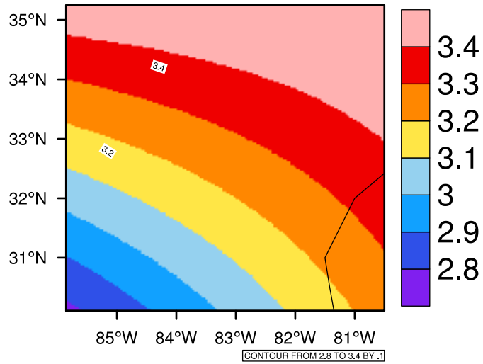
Yearly pr (mm/day) In 2070-2079 GFDL-ESM2M RCP85 - Georgia
