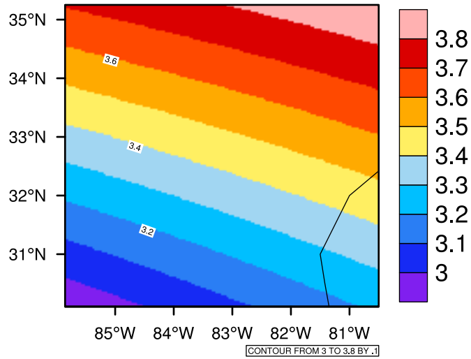
Yearly pr (mm/day) In 2080-2089 GFDL-ESM2M RCP85 - Georgia
