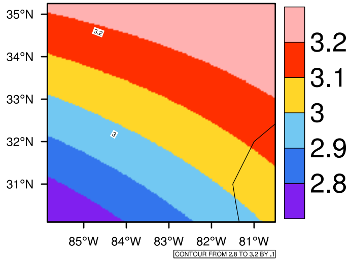
Yearly pr (mm/day) In 2090-2099 GFDL-ESM2M RCP85 - Georgia
