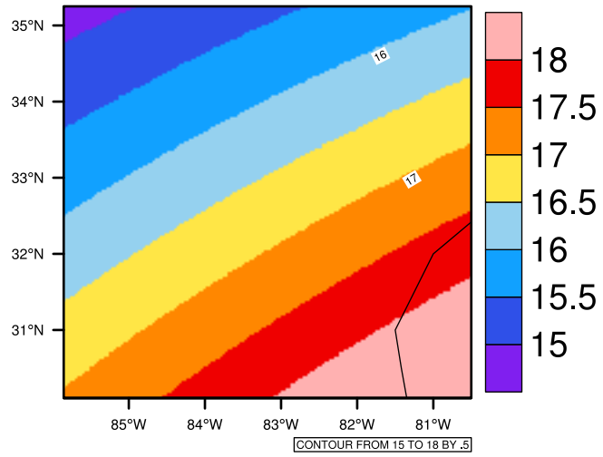
Yearly tas(c) In 1975-2005 GFDL-ESM2M historical - Georgia
