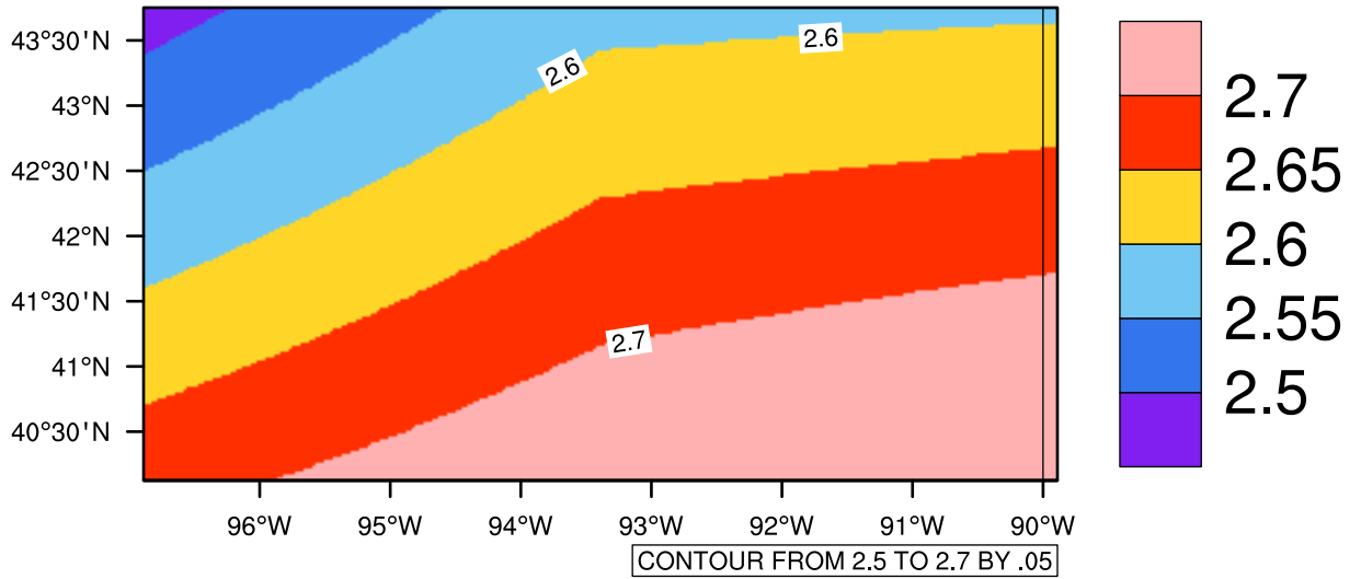
Yearly pr (mm/day) In 2020-2029 GFDL-ESM2M RCP45 - Iowa
