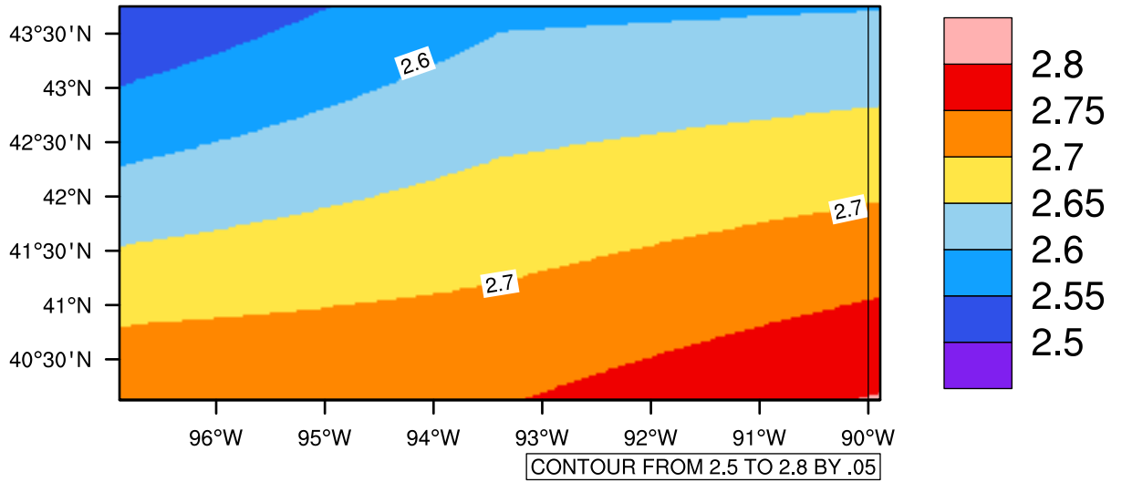
Yearly pr (mm/day) In 2040-2049 GFDL-ESM2M RCP45 - Iowa
