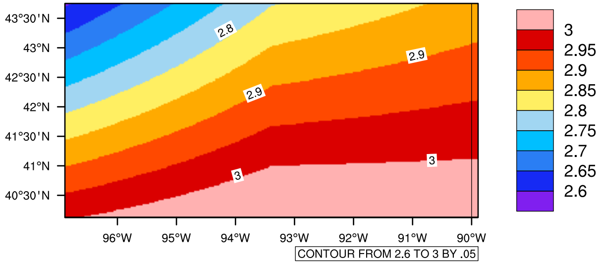
Yearly pr (mm/day) In 2050-2059 GFDL-ESM2M RCP45 - Iowa
