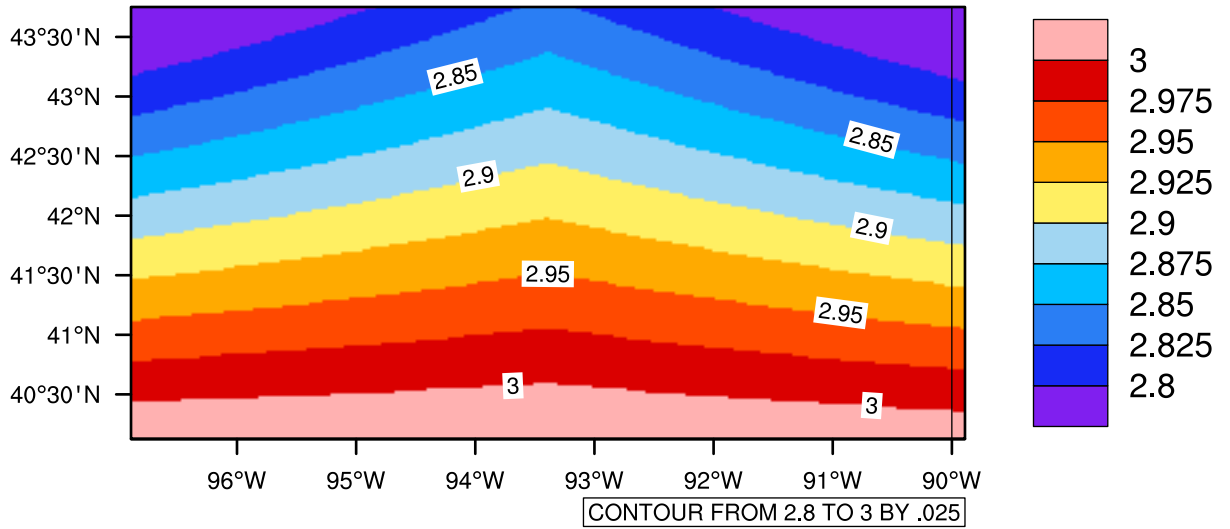
Yearly pr (mm/day) In 2060-2069 GFDL-ESM2M RCP45 - Iowa
