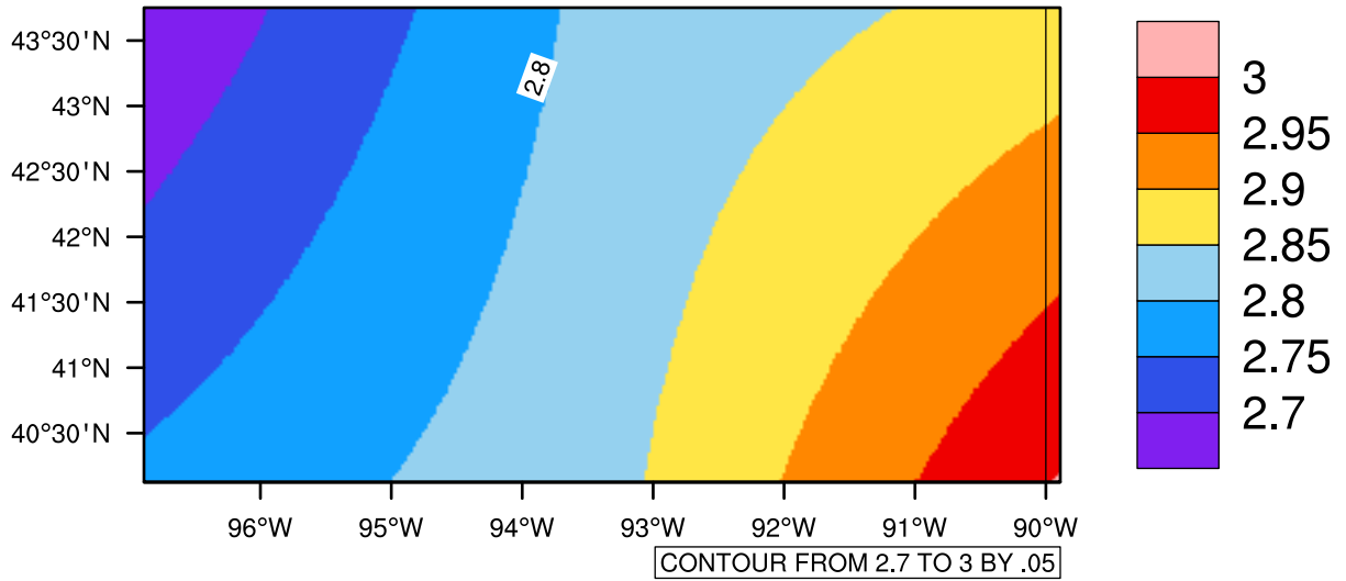
Yearly pr (mm/day) In 2070-2079 GFDL-ESM2M RCP45 - Iowa
