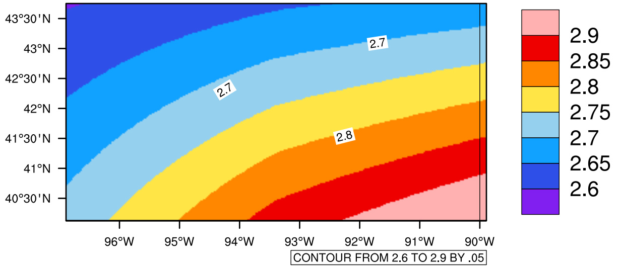
Yearly pr (mm/day) In 2080-2089 GFDL-ESM2M RCP45 - Iowa
