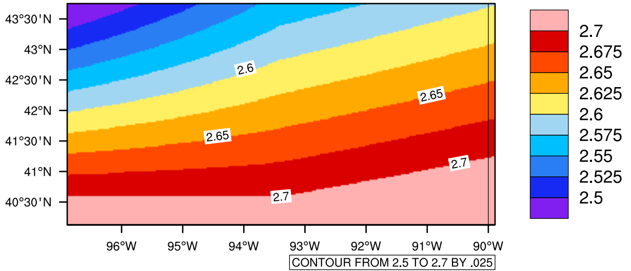
Yearly pr (mm/day) In 2030-2039 GFDL-ESM2M RCP85 - Iowa
