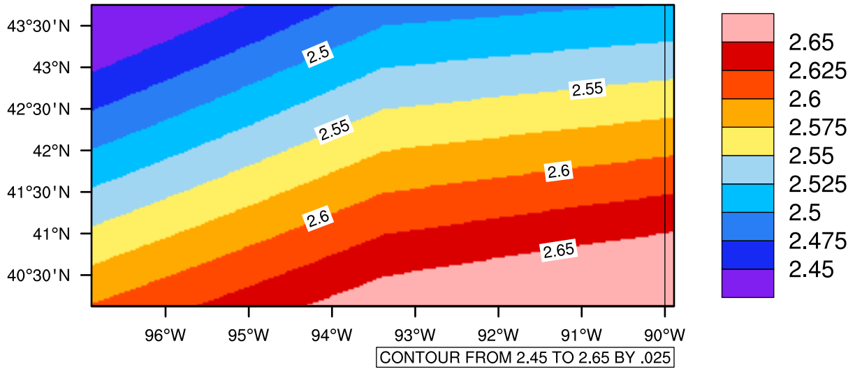
Yearly pr (mm/day) In 2050-2059 GFDL-ESM2M RCP85 - Iowa
