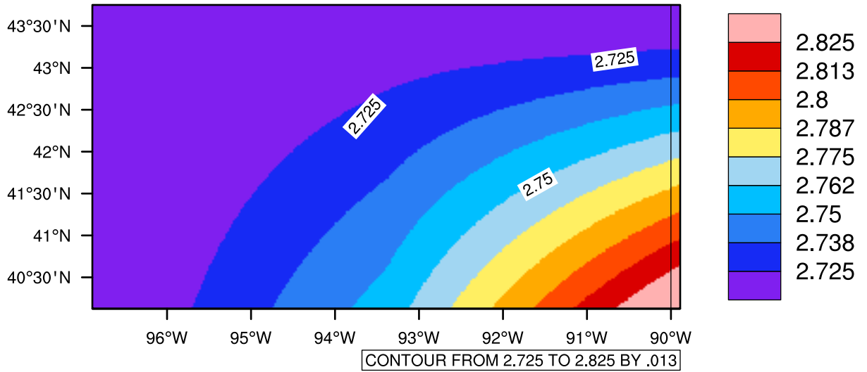
Yearly pr (mm/day) In 2070-2079 GFDL-ESM2M RCP85 - Iowa
