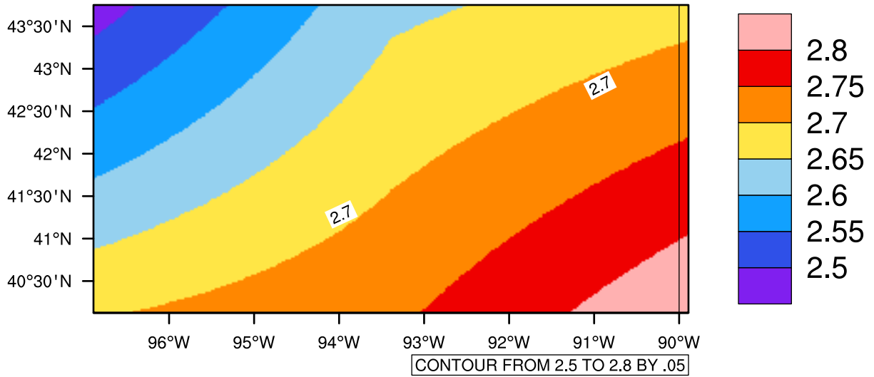
Yearly pr (mm/day) In 2090-2099 GFDL-ESM2M RCP85 - Iowa
