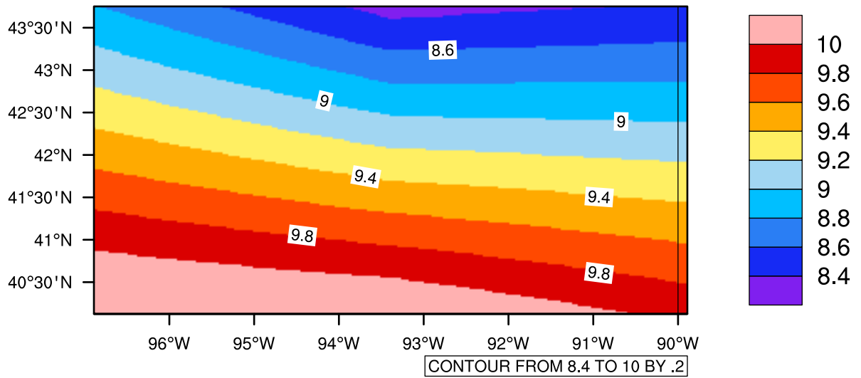
Yearly tas(c) In 2020-2029 GFDL-ESM2M RCP85 - Iowa
