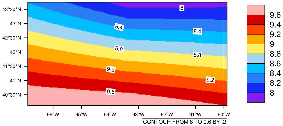
Yearly tas(c) In 1975-2005 GFDL-ESM2M historical - Iowa
