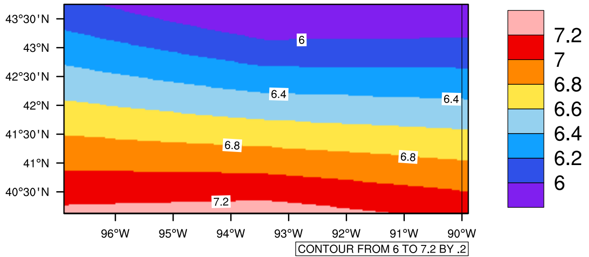
Yearly tasmin(c) In 2020-2029 GFDL-ESM2M RCP45 - Iowa
