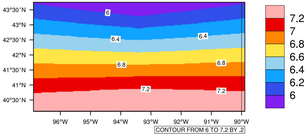
Yearly tasmin(c) In 2040-2049 GFDL-ESM2M RCP45 - Iowa
