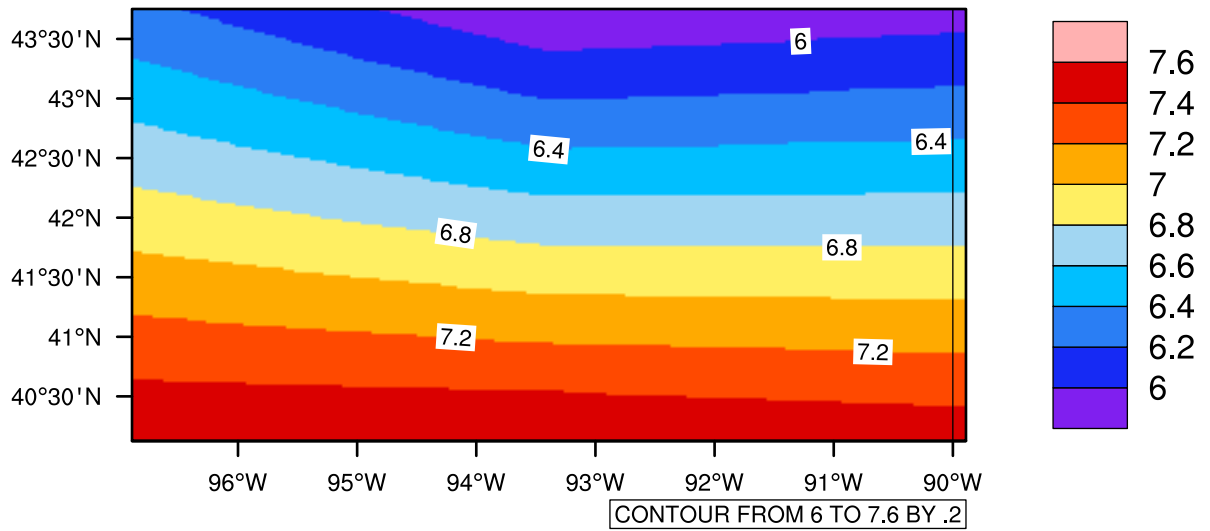
Yearly tasmin(c) In 2050-2059 GFDL-ESM2M RCP45 - Iowa
