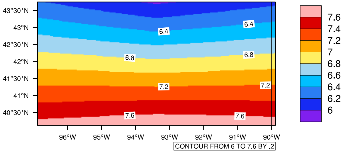
Yearly tasmin(c) In 2070-2079 GFDL-ESM2M RCP45 - Iowa
