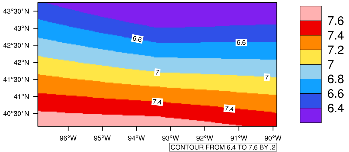
Yearly tasmin(c) In 2090-2099 GFDL-ESM2M RCP45 - Iowa
