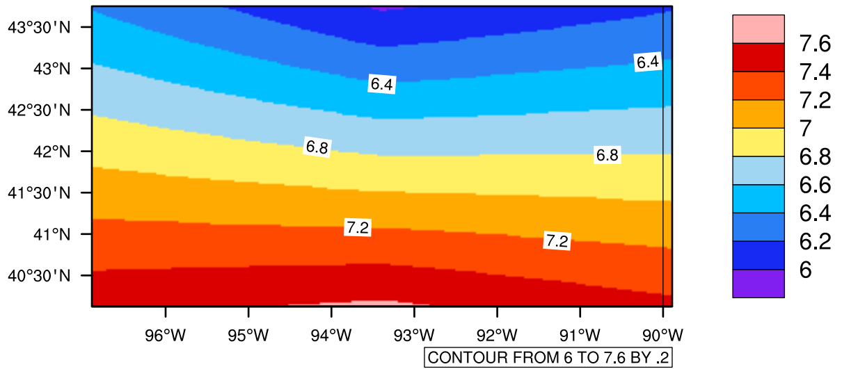
Yearly tasmin(c) In 2030-2039 GFDL-ESM2M RCP85 - Iowa
