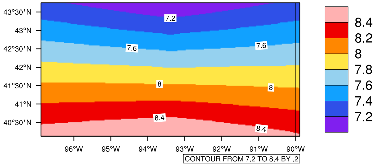
Yearly tasmin(c) In 2050-2059 GFDL-ESM2M RCP85 - Iowa
