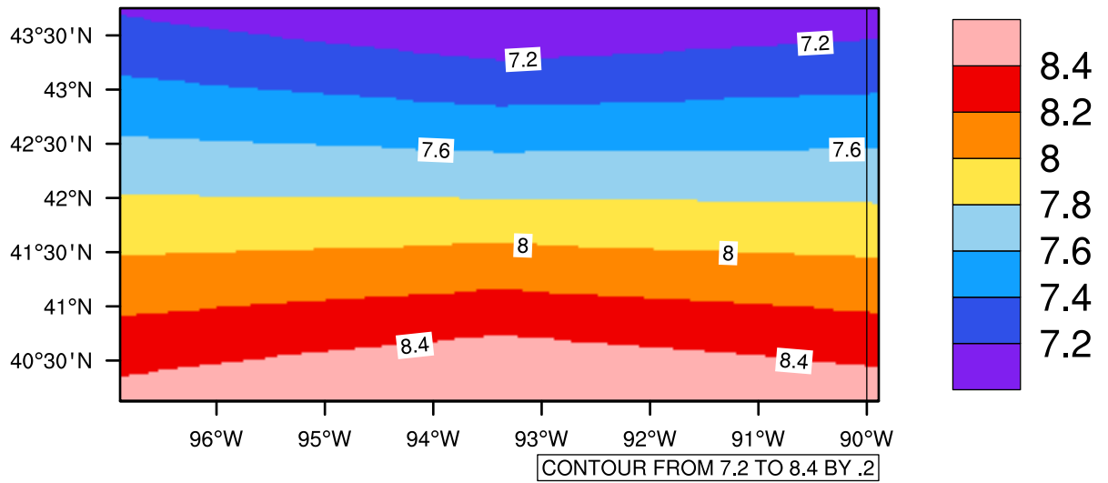
Yearly tasmin(c) In 2060-2069 GFDL-ESM2M RCP85 - Iowa
