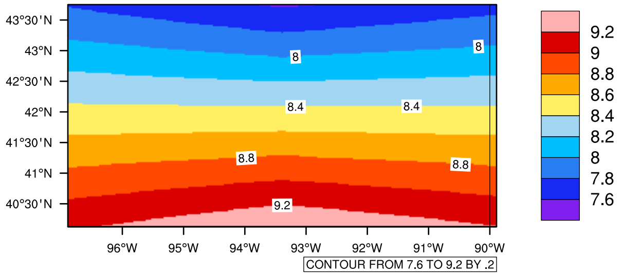
Yearly tasmin(c) In 2070-2079 GFDL-ESM2M RCP85 - Iowa
