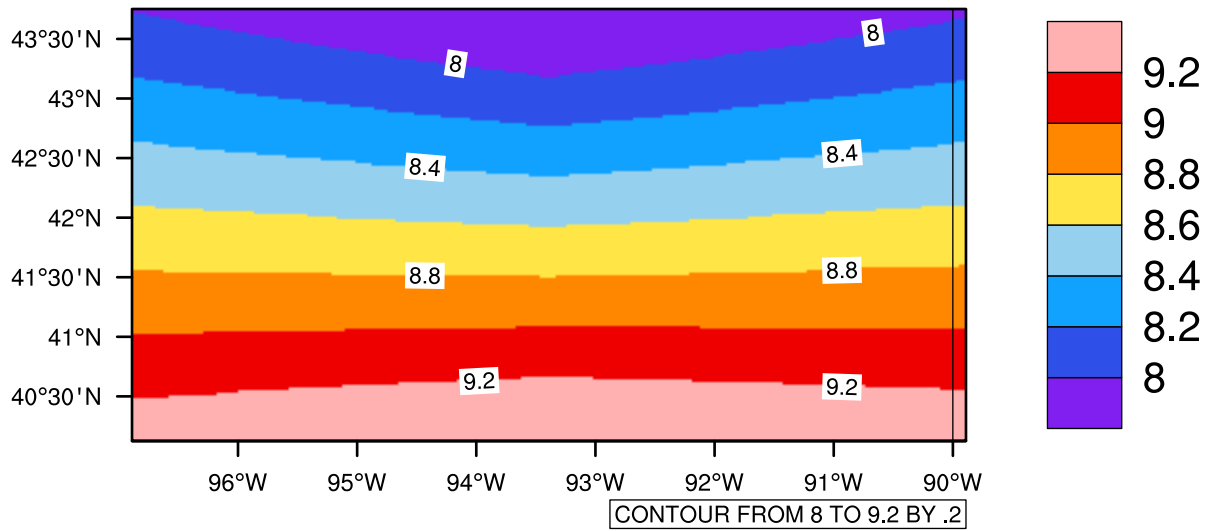
Yearly tasmin(c) In 2080-2089 GFDL-ESM2M RCP85 - Iowa
