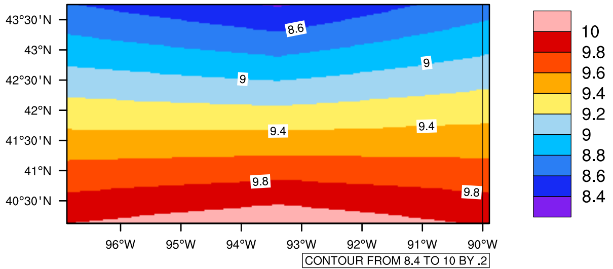
Yearly tasmin(c) In 2090-2099 GFDL-ESM2M RCP85 - Iowa
