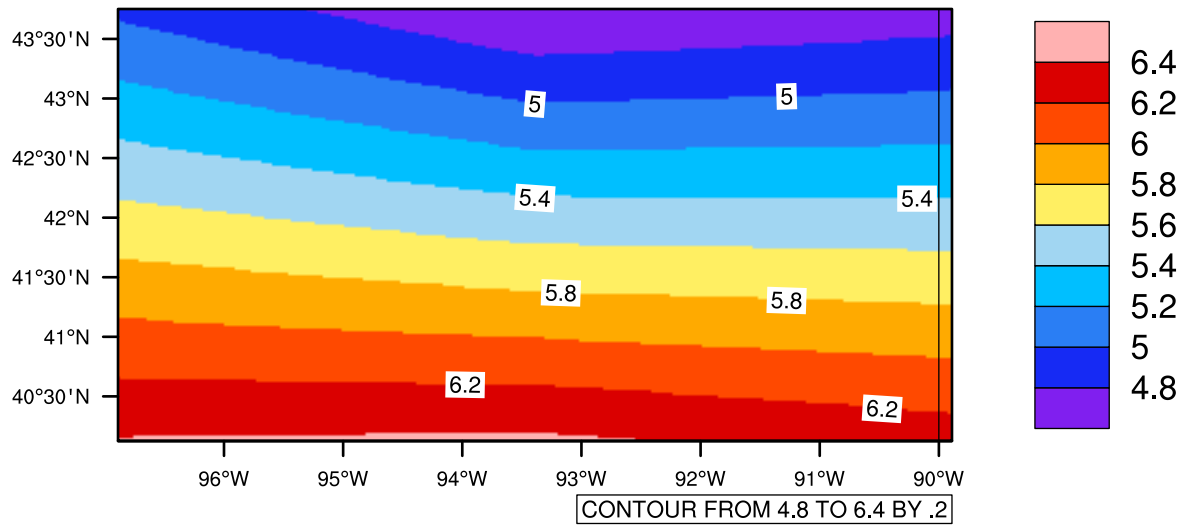
Yearly tasmin(c) In 1975-2005 GFDL-ESM2M historical - Iowa
