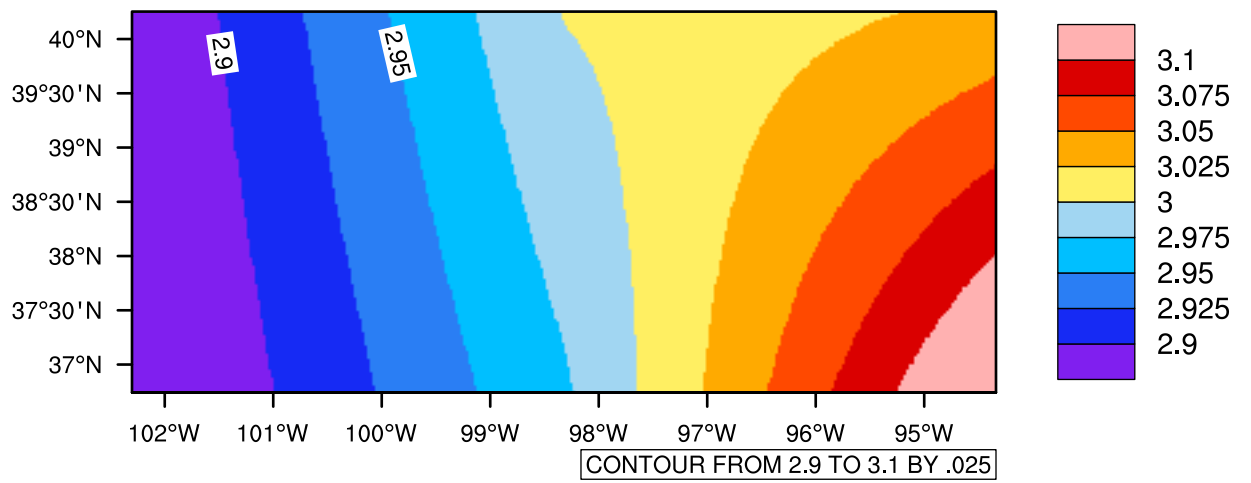
Yearly pr (mm/day) In 2040-2049 GFDL-ESM2M RCP85 - Kansas
