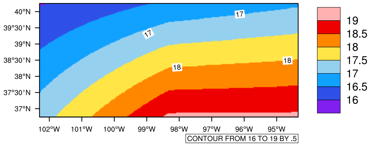
Yearly tasmx(c) In 2020-2029 GFDL-ESM2M RCP45 - Kansas
