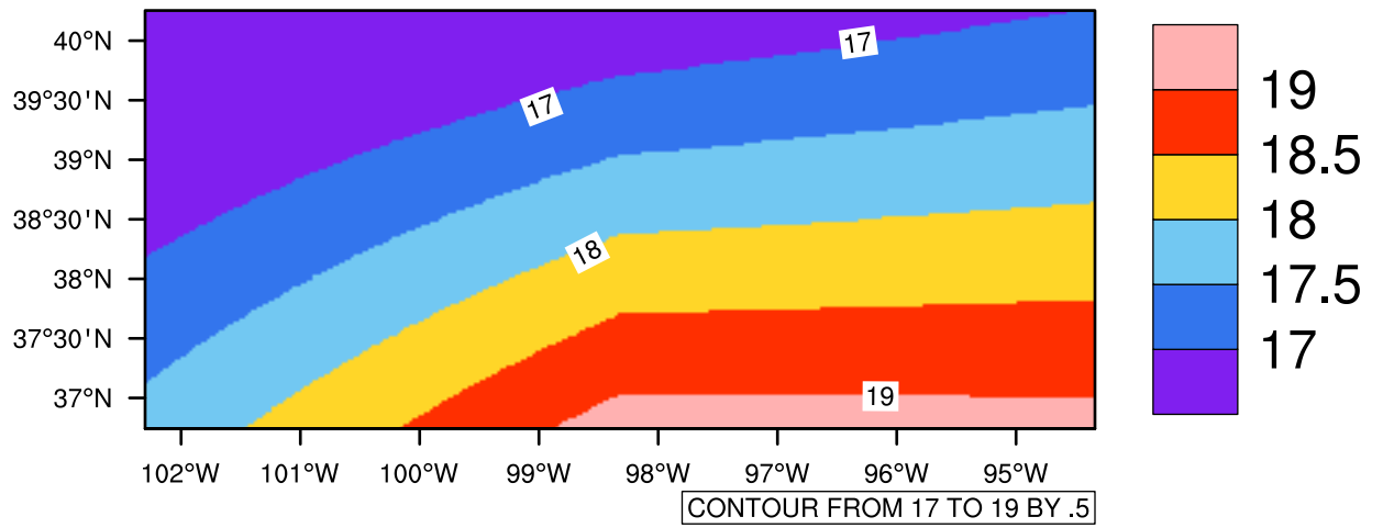
Yearly tasmx(c) In 2030-2039 GFDL-ESM2M RCP45 - Kansas
