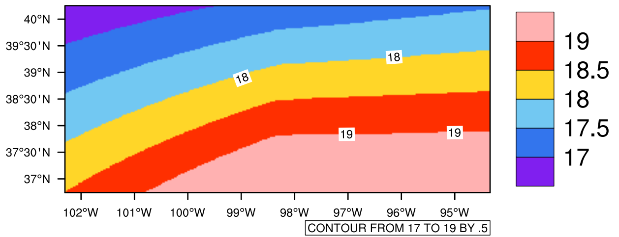
Yearly tasmx(c) In 2040-2049 GFDL-ESM2M RCP45 - Kansas
