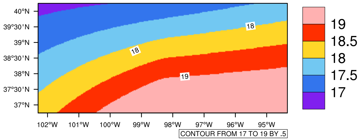
Yearly tasmx(c) In 2070-2079 GFDL-ESM2M RCP45 - Kansas
