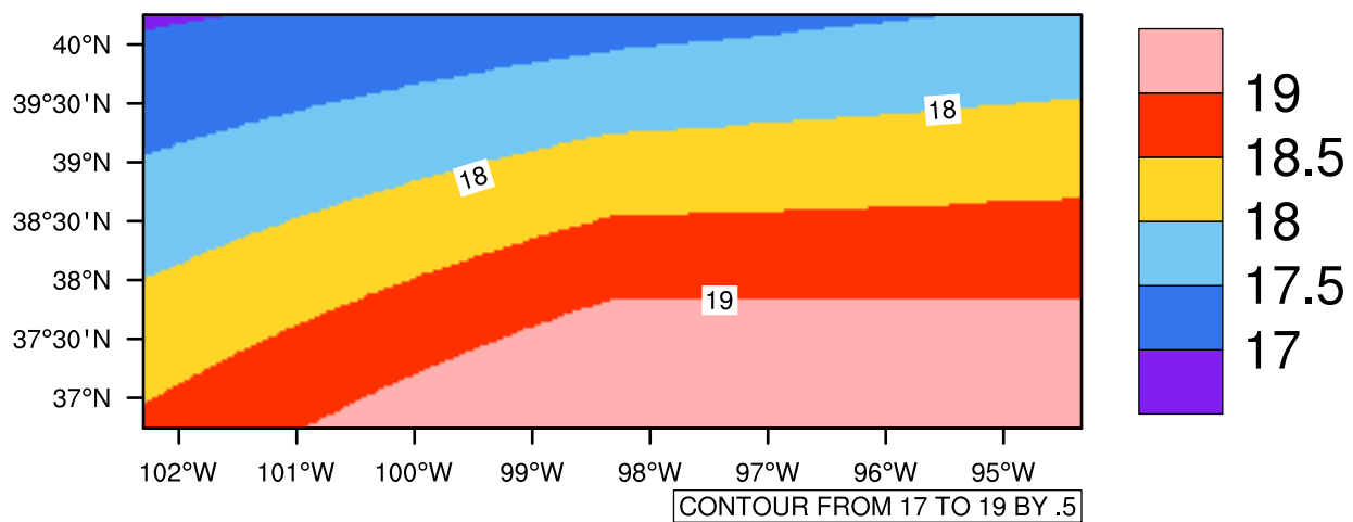
Yearly tasmx(c) In 2090-2099 GFDL-ESM2M RCP45 - Kansas
