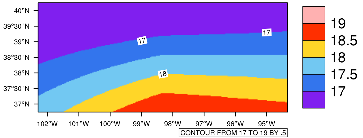
Yearly tasmx(c) In 2020-2029 GFDL-ESM2M RCP85 - Kansas
