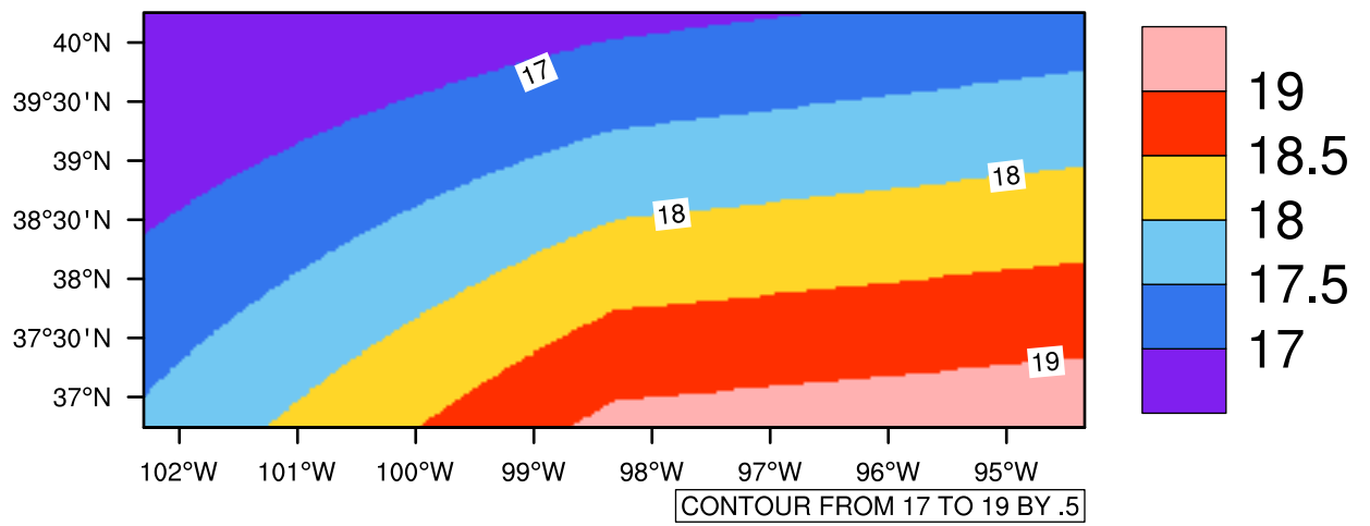
Yearly tasmx(c) In 2030-2039 GFDL-ESM2M RCP85 - Kansas
