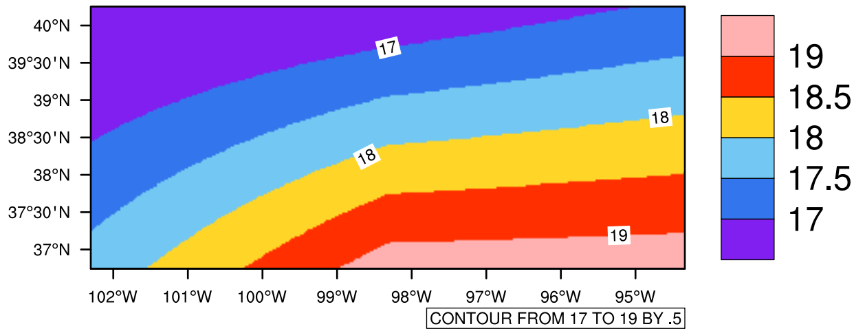
Yearly tasmx(c) In 2040-2049 GFDL-ESM2M RCP85 - Kansas
