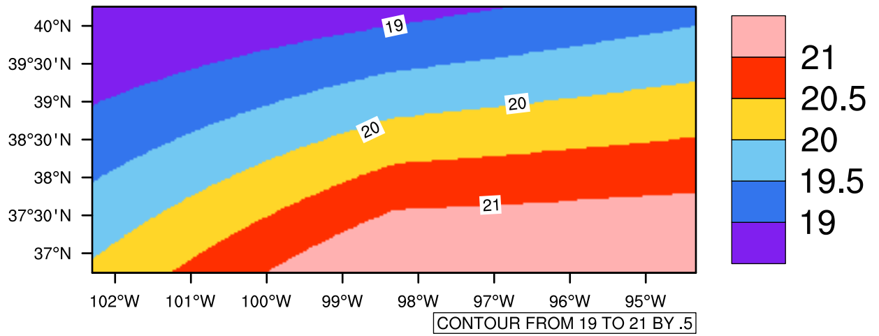
Yearly tasmx(c) In 2080-2089 GFDL-ESM2M RCP85 - Kansas
