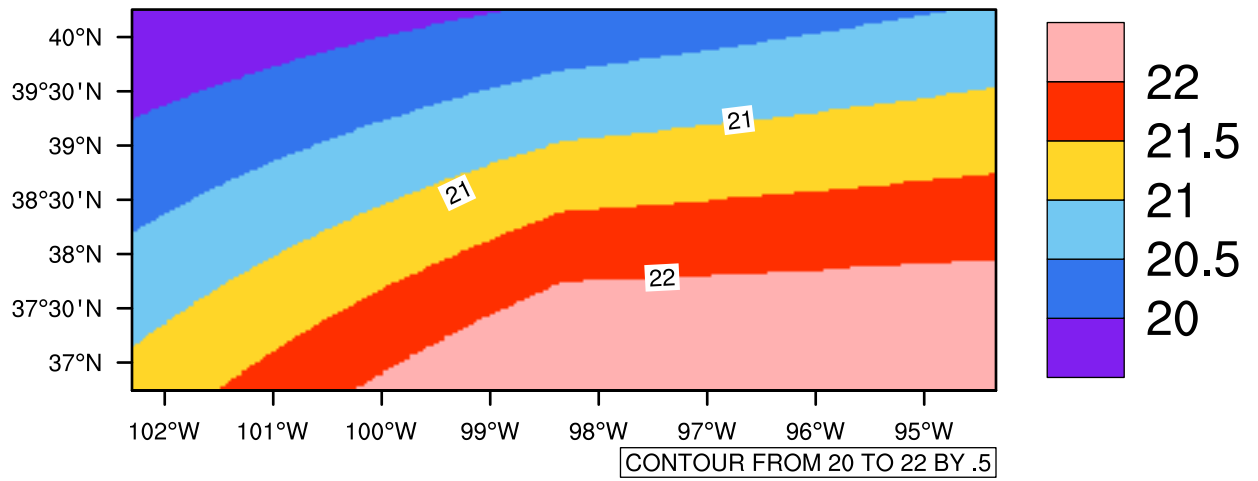
Yearly tasmx(c) In 2090-2099 GFDL-ESM2M RCP85 - Kansas
