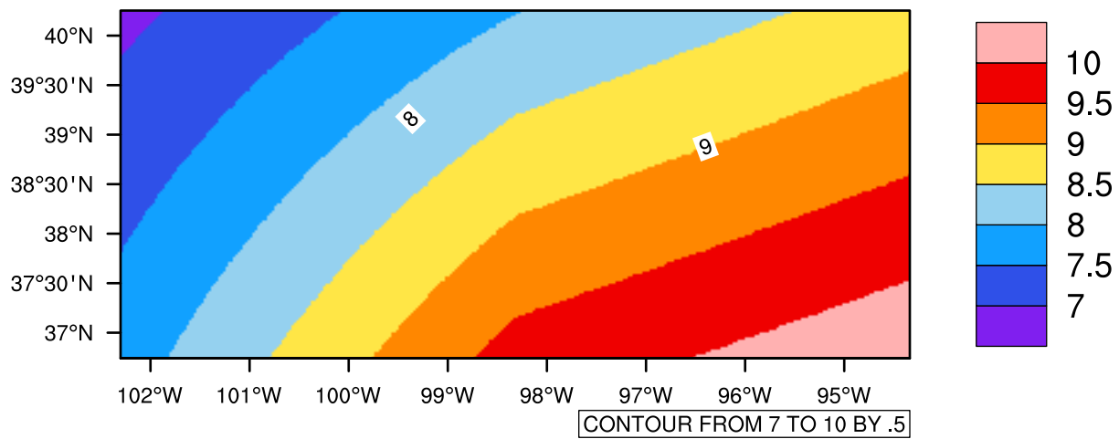
Yearly tasmin(c) In 2020-2029 GFDL-ESM2M RCP45 - Kansas
