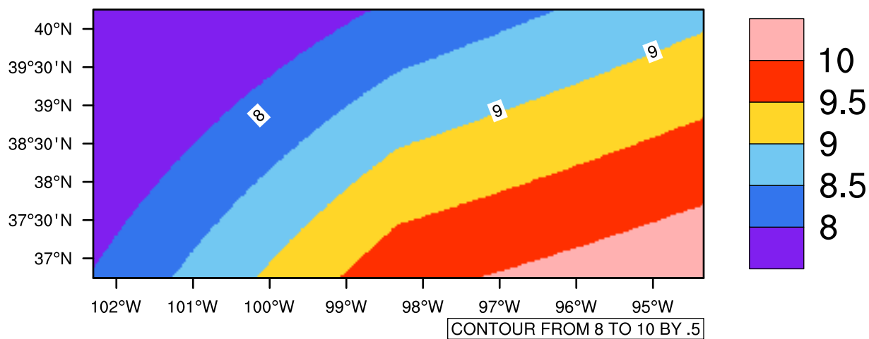
Yearly tasmin(c) In 2030-2039 GFDL-ESM2M RCP45 - Kansas
