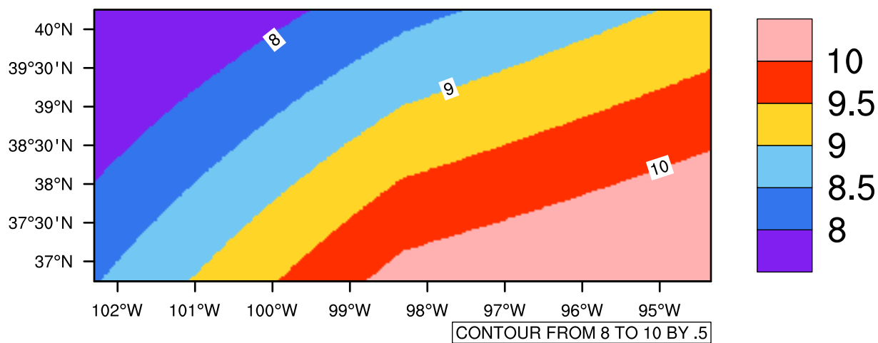
Yearly tasmin(c) In 2040-2049 GFDL-ESM2M RCP45 - Kansas
