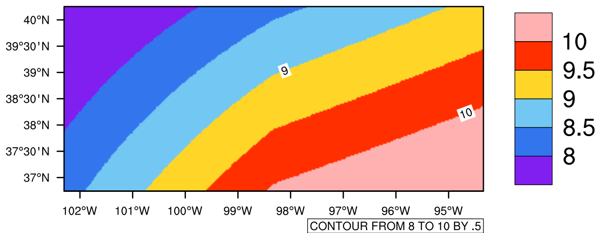
Yearly tasmin(c) In 2050-2059 GFDL-ESM2M RCP45 - Kansas
