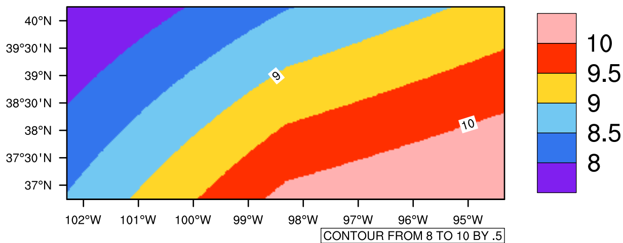
Yearly tasmin(c) In 2090-2099 GFDL-ESM2M RCP45 - Kansas
