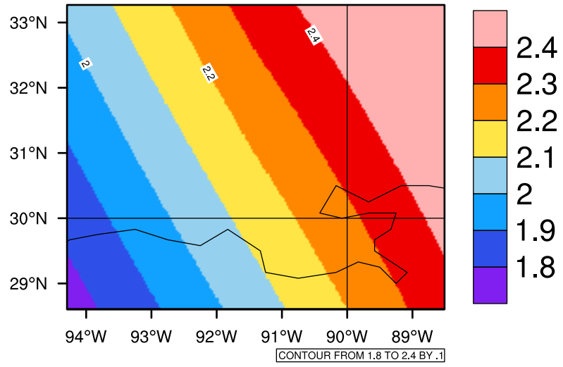
Yearly pr (mm/day) In 2050-2059 GFDL-ESM2M RCP45 - Louisiana
