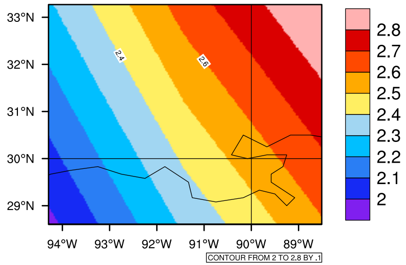
Yearly pr (mm/day) In 2080-2089 GFDL-ESM2M RCP45 - Louisiana
